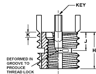
Self-Locking
